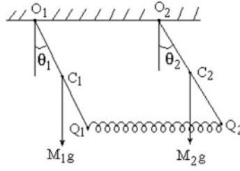
Figure 6.2.1 The coupled pendulum.
