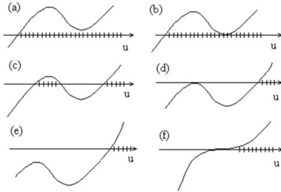
Figure 4.4.1 Schematic graphs of the function f(u) .
